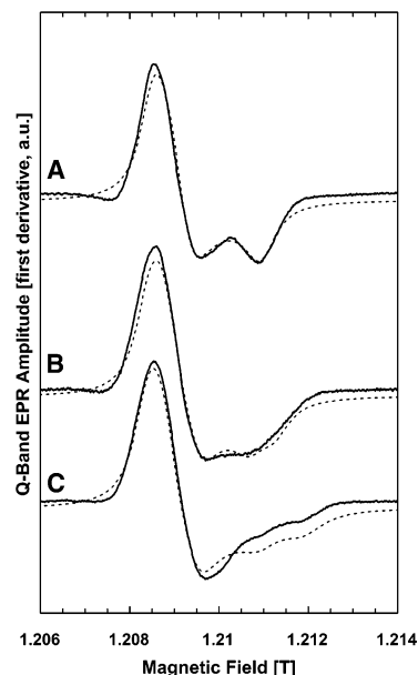
FIGURE 5: Q-band (34 GHz) EPR spectra of \text{bo}_3 -QOX under reducing conditions. From top to the bottom: (A) reconstituted with unlabeled UQ-2 ( ^{12}\text{C} ), (B) reconstituted with UQ-2 ^{13}\text{C} -labeled at the 1-carbonyl position, and (C) reconstituted with UQ-2 ^{13}\text{C} -labeled at the 4-carbonyl position. Experimental conditions: MW power = 1.2 \times 10^{-3} mW; field modulation frequency = 100 kHz, field modulation amplitude = 3 G; T = 80 K; and microwave frequency = 33.98 GHz. Spectral simulations are performed using the \mathbf{g} tensor given in the text, Table 1, ref 13, and a line width of 3.5 G.
