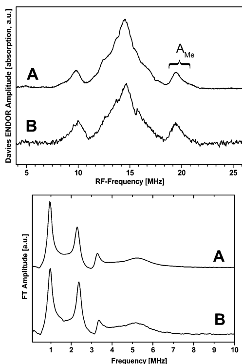
FIGURE 3: Davies ^1\text{H} -ENDOR (top) and Fourier transformed 3 pulse ESEEM (bottom) spectra of the \text{bo}_3 -QOX of E. coli under reducing conditions. (A) Native UQ-8 and (B) after reconstitution with ^{12}\text{C} -UQ-2. Experimental conditions: Davies ^1\text{H} -ENDOR; microwave \pi -pulse length = 200 ns; radio frequency \pi -pulse length = 9 \mu\text{s} ; and temperature = 20 K. Frequency domain 3-pulse ESEEM spectra: microwave \pi/2 -pulse length = 8 ns; \tau = 200 ns; and temperature = 20 K.
