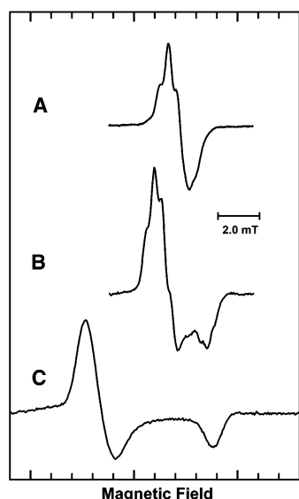
FIGURE 4: CW-EPR spectra of \text{Q}_\text{H}^{\bullet-} taken at (A) X-band (9.47 GHz), (B) Q-band (34.0 GHz), and (C) W-band (94.0 GHz) using a field modulation amplitude of 0.5 G at T = 80 K. For all other experimental conditions, see Figures 2, 4, and 5.
